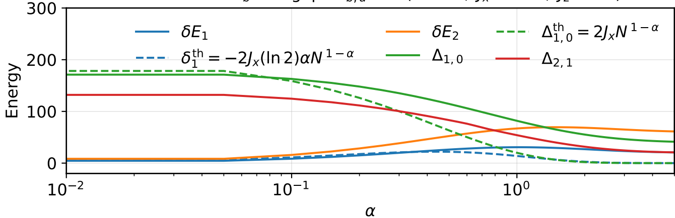
Band widths \delta E_b and gaps \Delta_{b,d} vs \alpha ( N = 10, J_x = 10.0, J_z = 1.0 )
